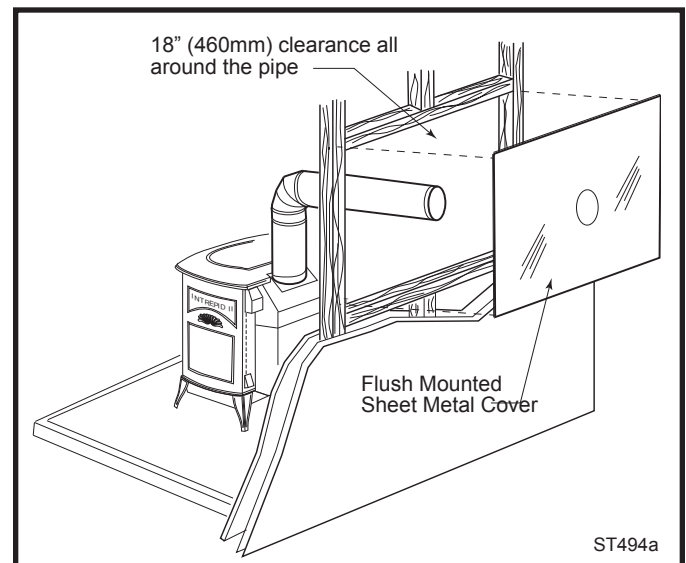
Fig. 10 An approved wall pass-through for Canada.
