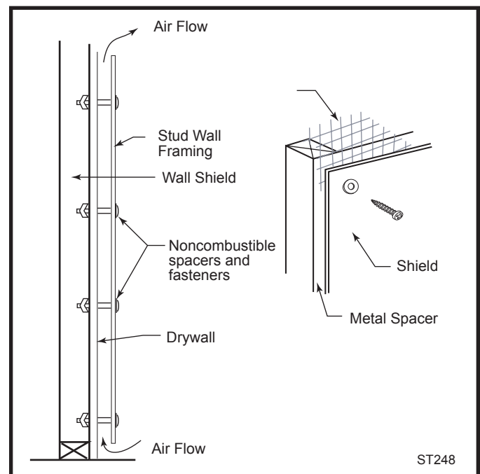
Fig. 13 Approved wall shield construction.
