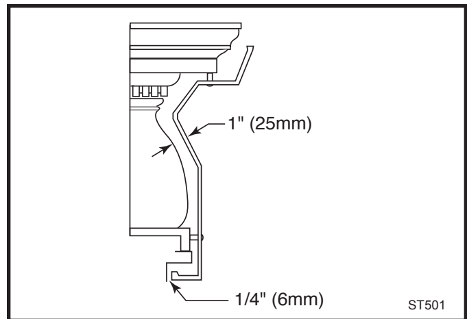
Fig. 14 A custom-formed mantel shield.
