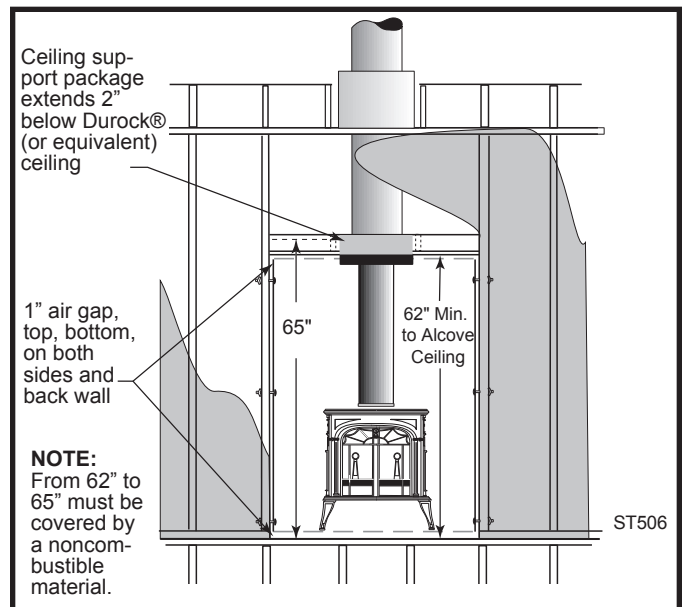
Fig. 20 Front view: 65" minimum clearance from hearth to combustibles on front face. Combustible facing may overlap metal studs by only 1". It should not extend below the height of the noncombustible ceiling.
