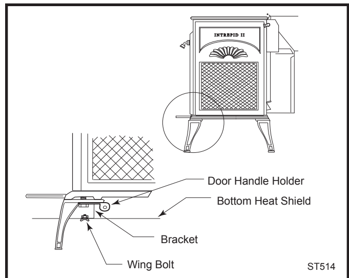
Fig. 29 Handle holder and heat shield positions.
