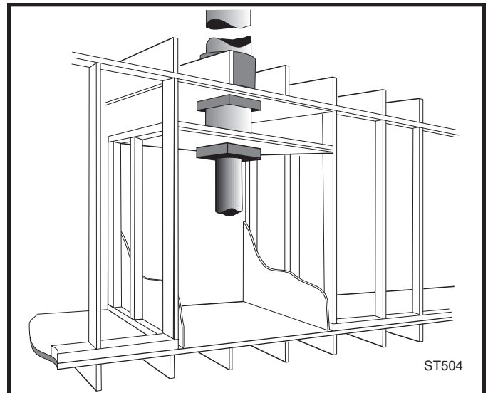
Fig. 18 Cutaway perspective of alcove installation.
