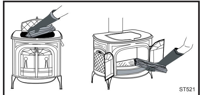
Fig. 36 Top loading is the best way to add fuel during regular use. Front loading is useful for kindling a fire.
