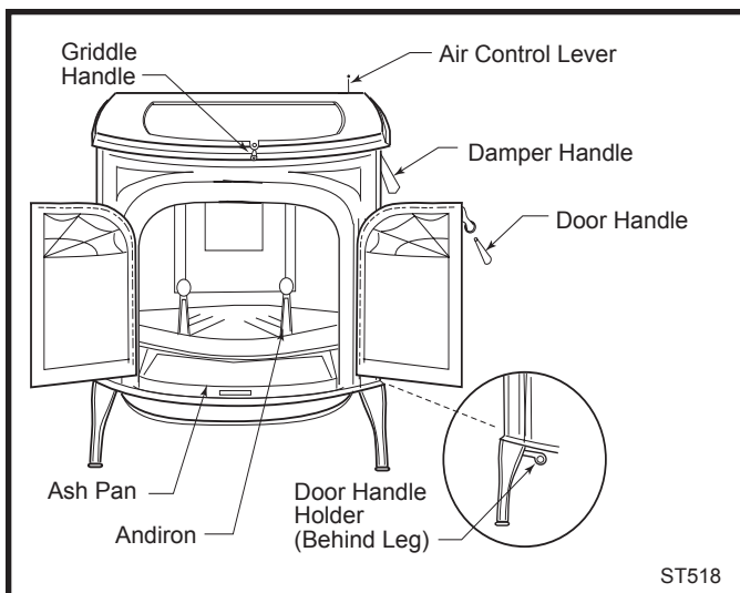
Fig. 32 The Intrepid II controls.
