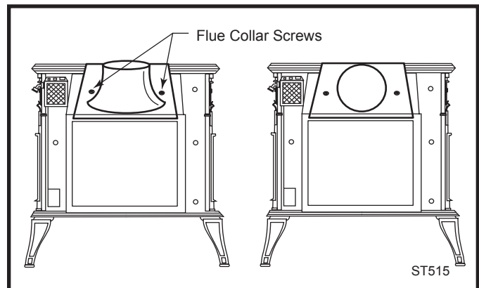
Fig. 30 Reversing the flue collar.
