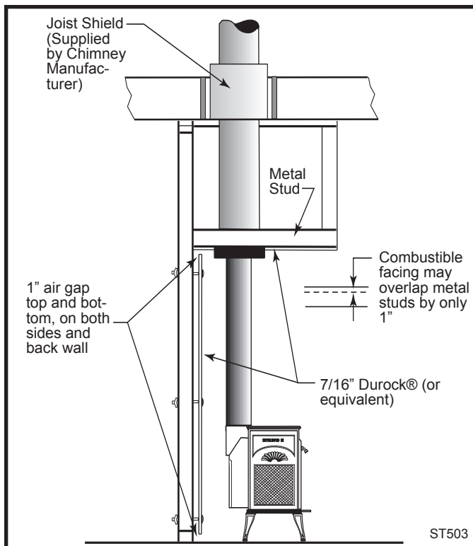
Fig. 17 Alcove side section.
