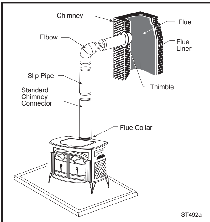
Fig. 6 Chimney connection in a freestanding installation.
