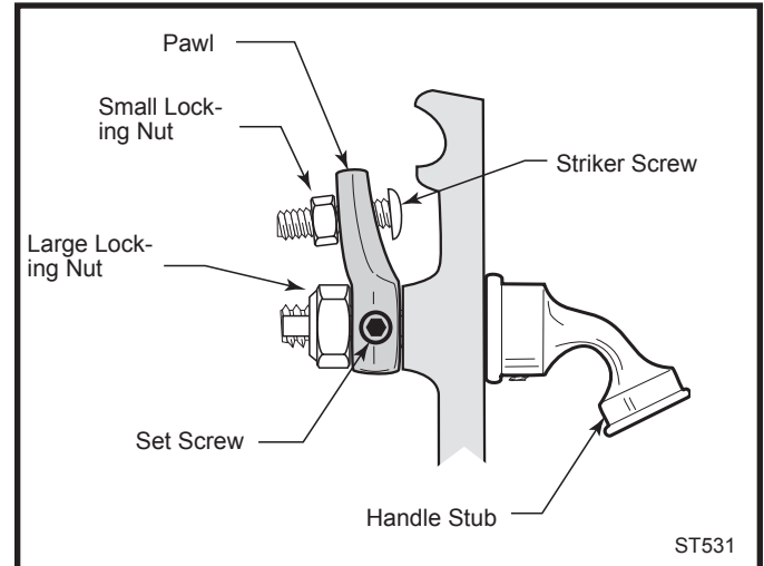
Fig. 44 Turn the door latch striker screw in or out to tighten or loosen the door latch.
