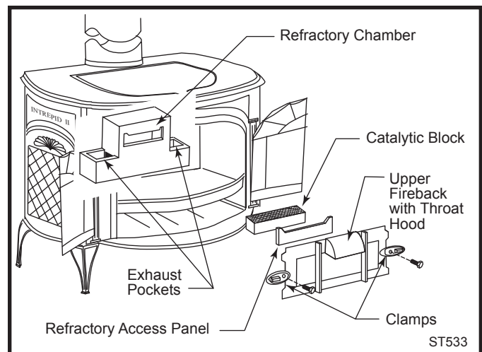
Fig. 46 Removing the catalytic element.
