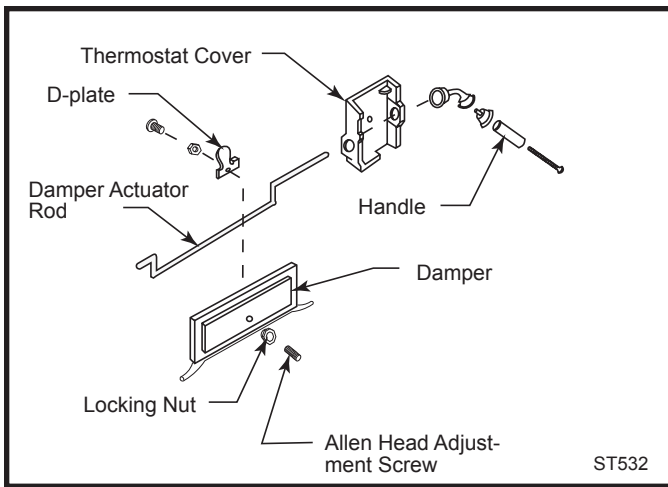
Fig. 45 Tighten the damper adjustment screw for a snug seal.
