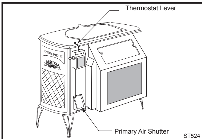
Fig. 43 The primary air shutter must move freely.
