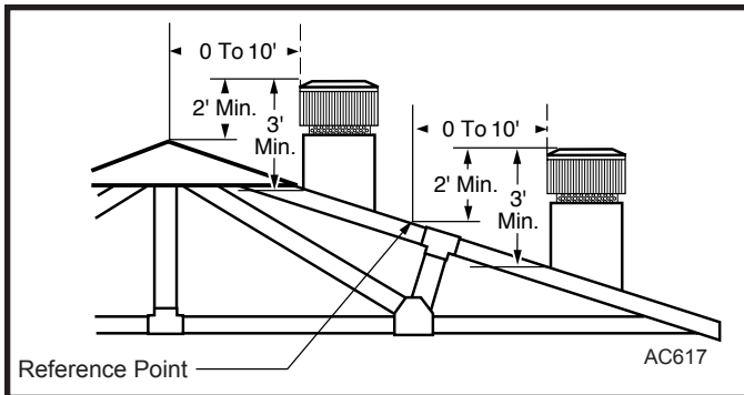
Fig. 3 The 2'-3'-10' Chimney Rule.
