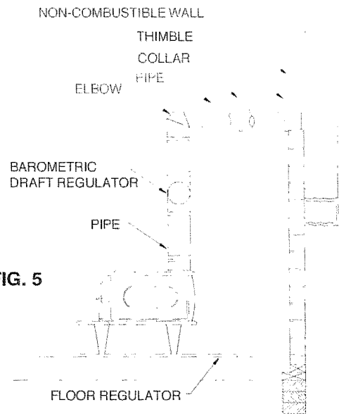
FLUE CONNECTION-NON-COMBUSTIBLE WALL
