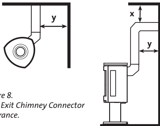
Figure 7. Floor protection dimensions.
