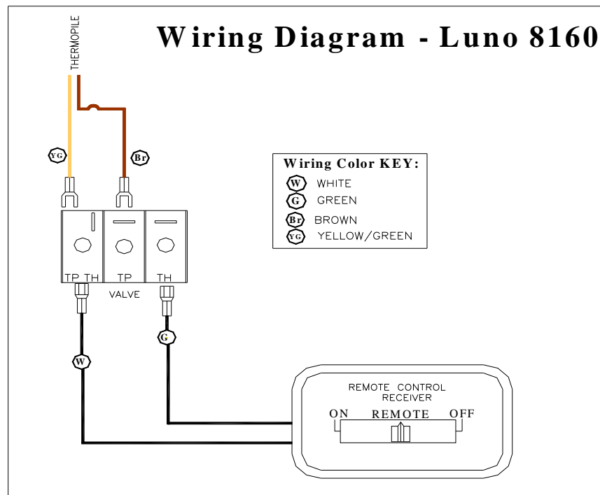
Figure 5: Luno 8160 Wiring Diagram
