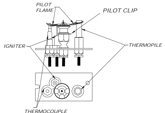
Figure 8: Pilot flame and assembly
