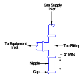
Figure 7: Typical Sediment Trap (required in all installations)
