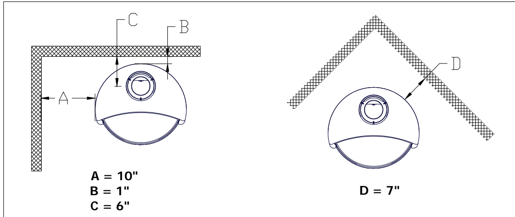
Figure 3 - Clearance to Combustibles
