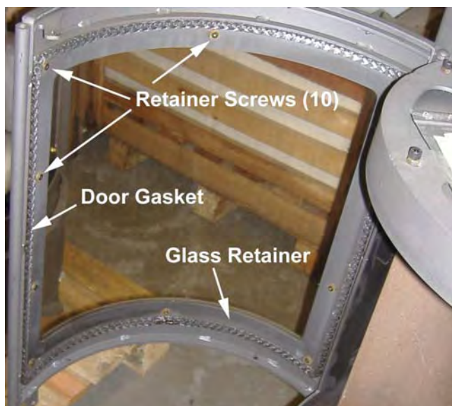
Figure 10: Door assembly
