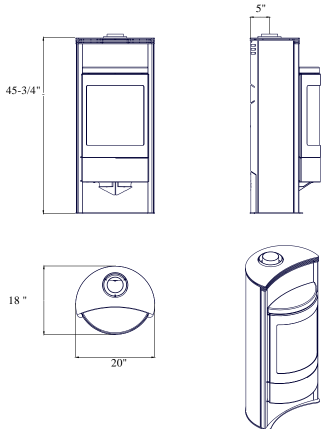
Figure 1 – Luno Dimensions
