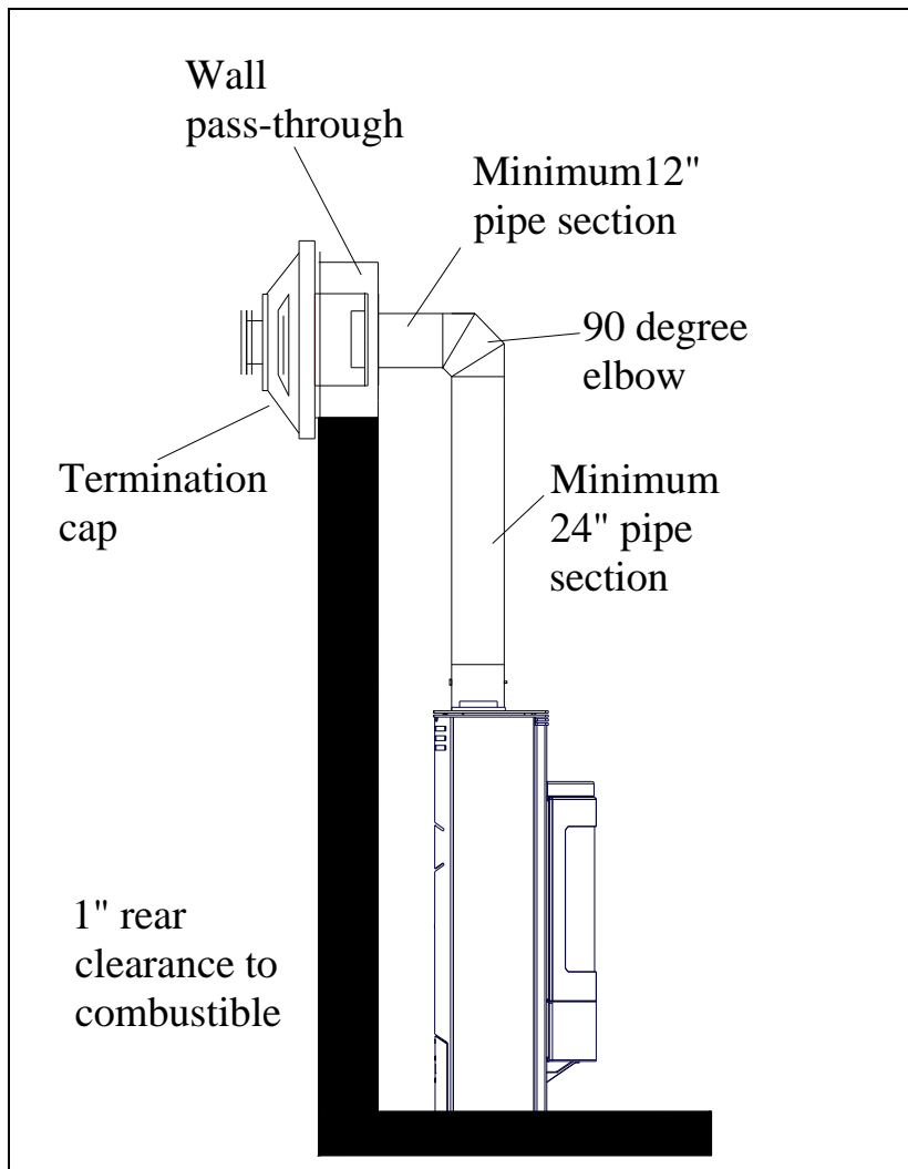
Figure 4 - Minimum Vent Configuration and Clearances
