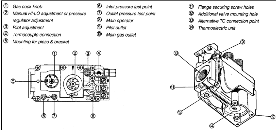
Figure 6: Gas Control Valve
