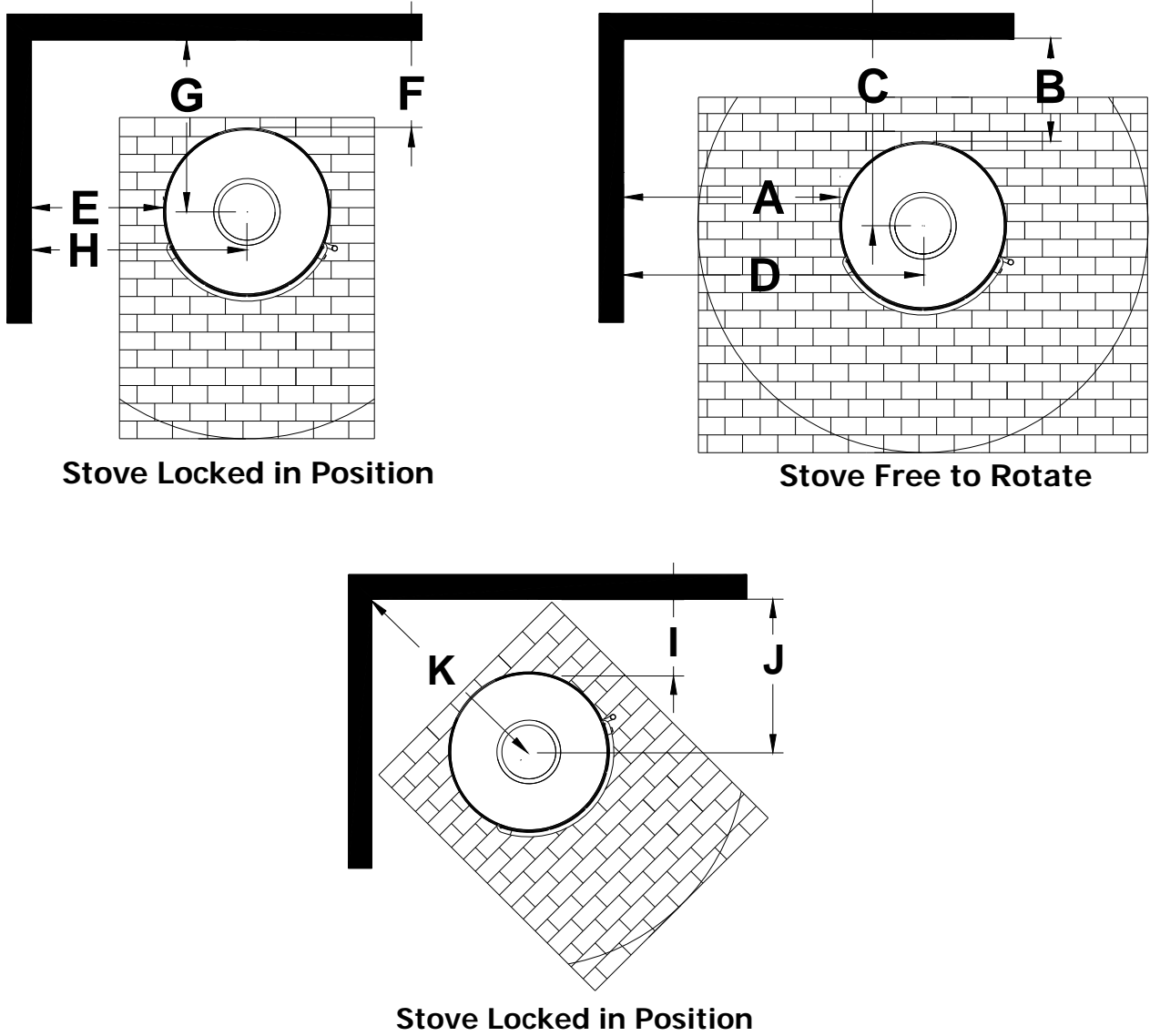
Figure 8 Clearance to combustibles
