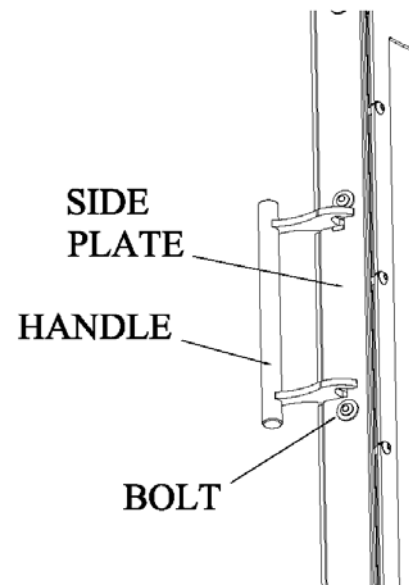
Figure 11 Handle Assembly Detail
