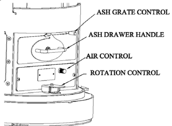
Figure 9 Controls
