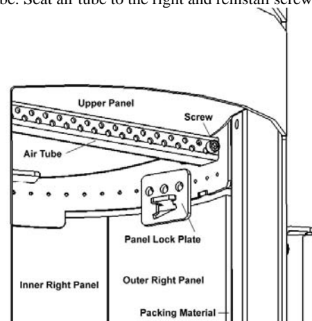
Figure 13 - Panel Detail
