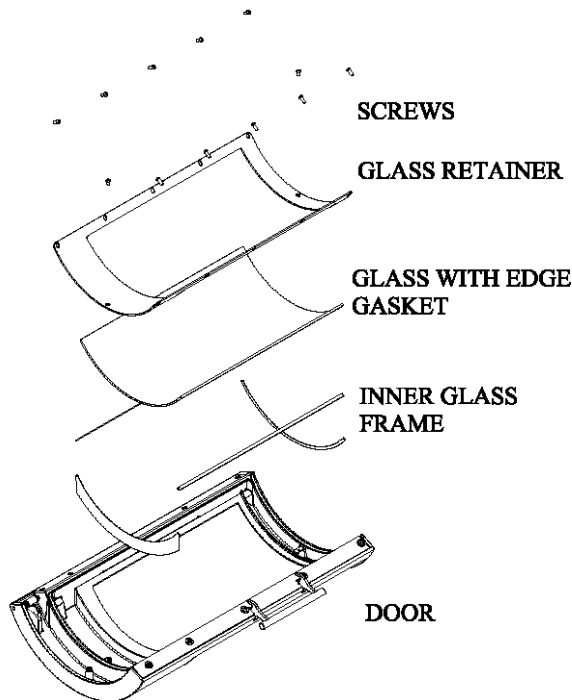
Figure 12 Glass Assembly
