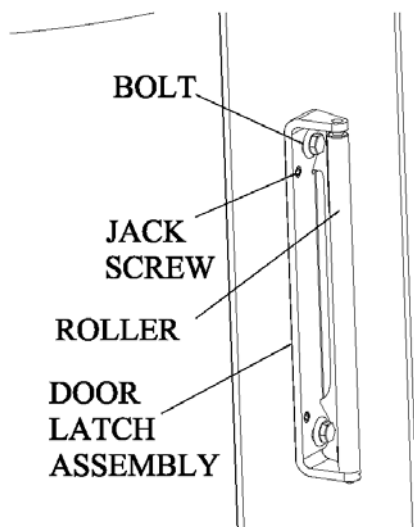
Figure 10 Latch Assembly Detail
