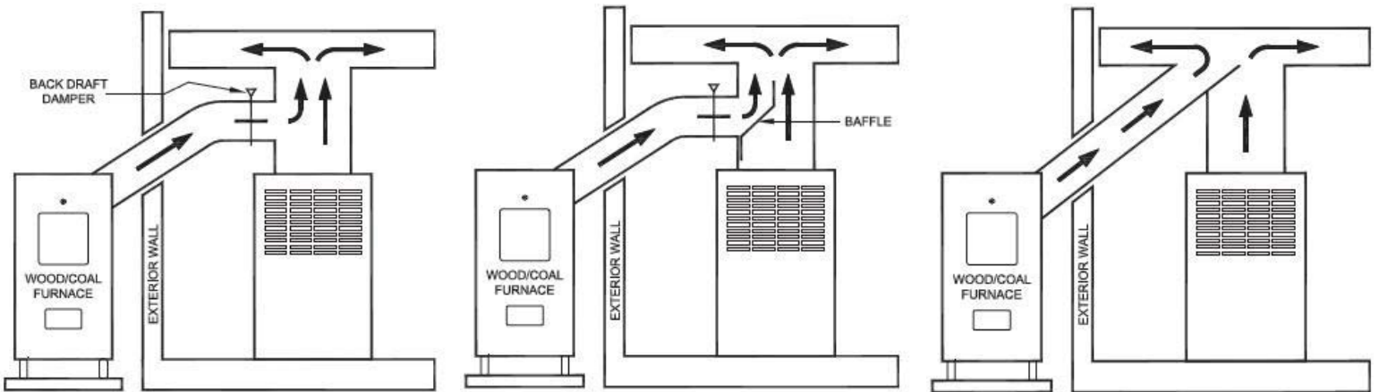
Ductwork Method #1
