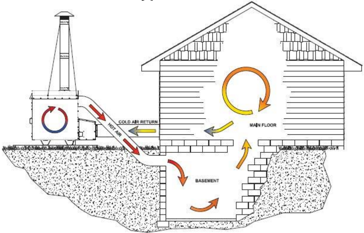
1600EF - No Ductwork Installation
