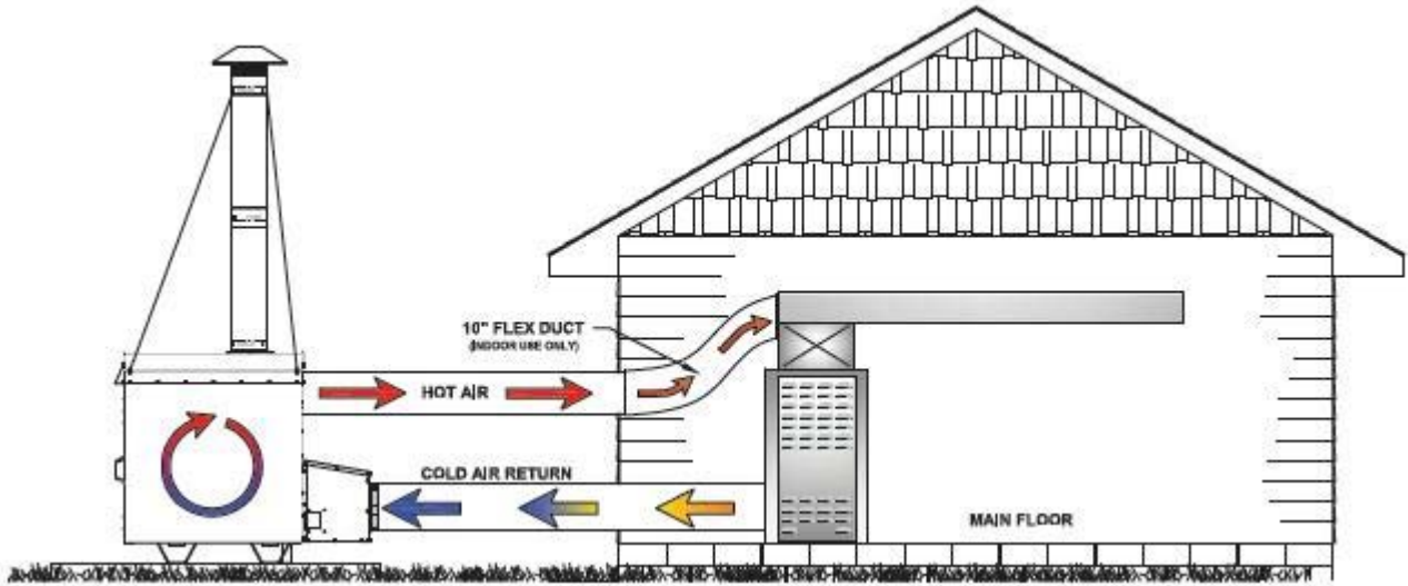
1600EF - Ductwork Installation
